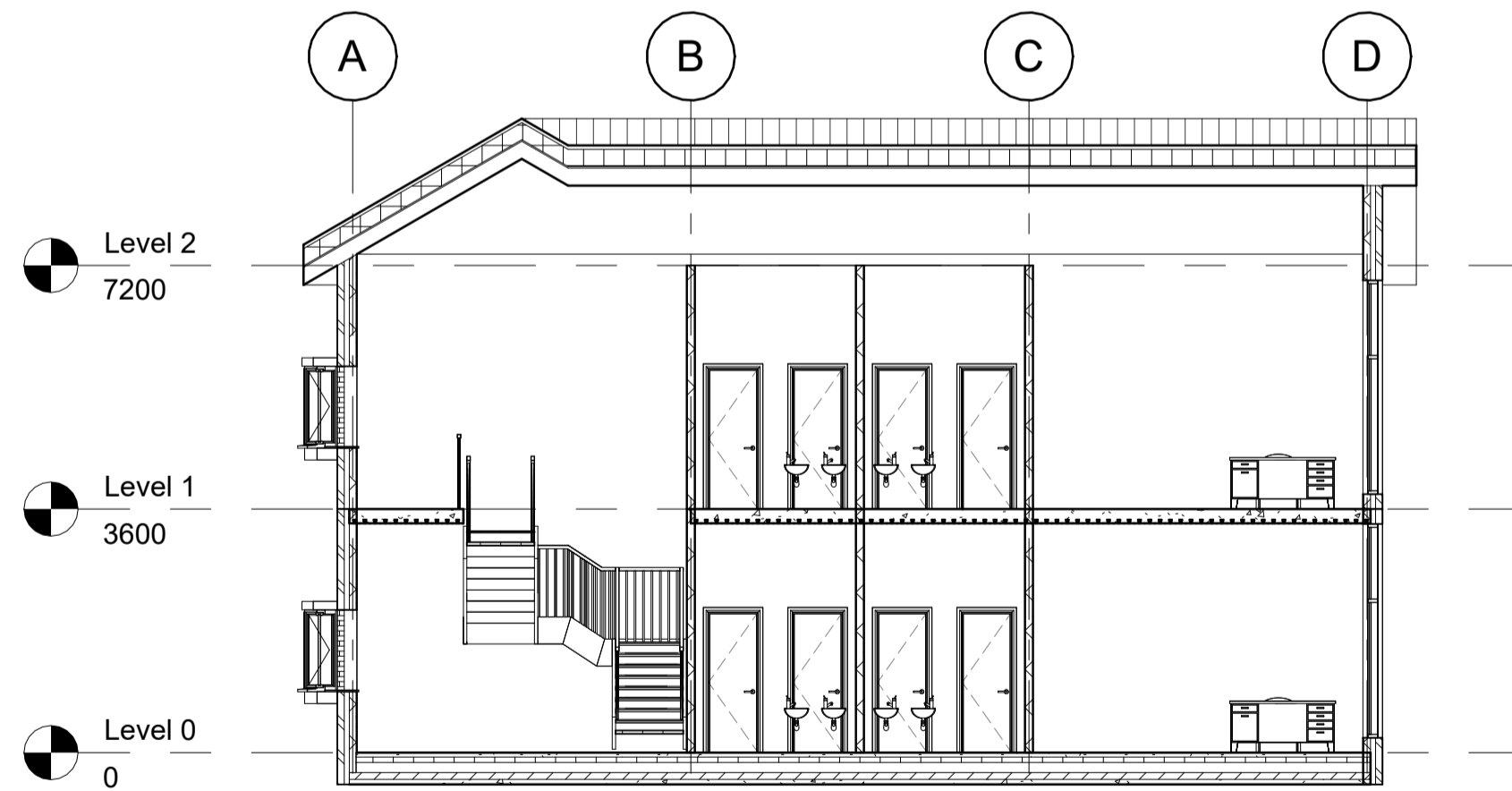
2 Side View 2 1 : 100
