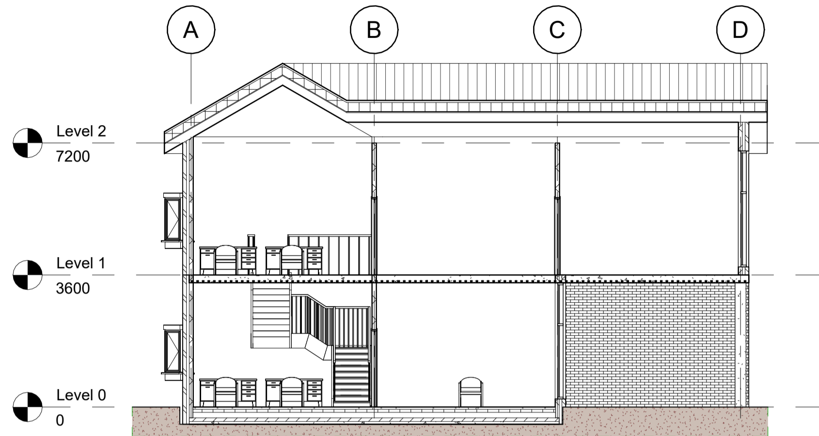
1 Side View 1 1 : 100
